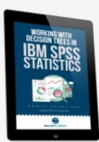
Working with decision trees in SPSS Statistics
