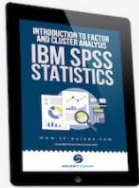
Factor and Cluster Analysis with IBM SPSS Statistics
